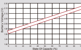
Relationship of OCV And State of Charge(20°C)
