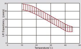
Effect of Temperature on Long Term Life
