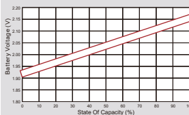
Relationship of OCV And State of Charge(20°C)
